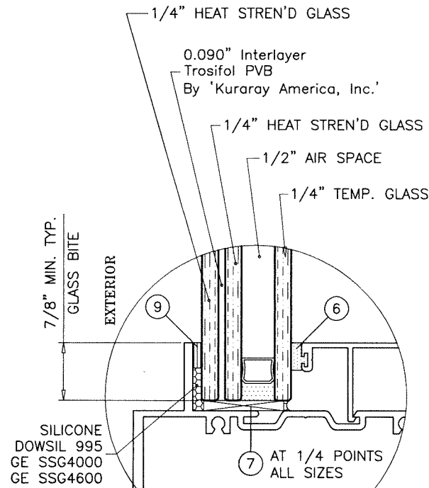
GLASS TYPE 'Di' 1-3/8" OVERALL LAM. INSUL. GLASS
