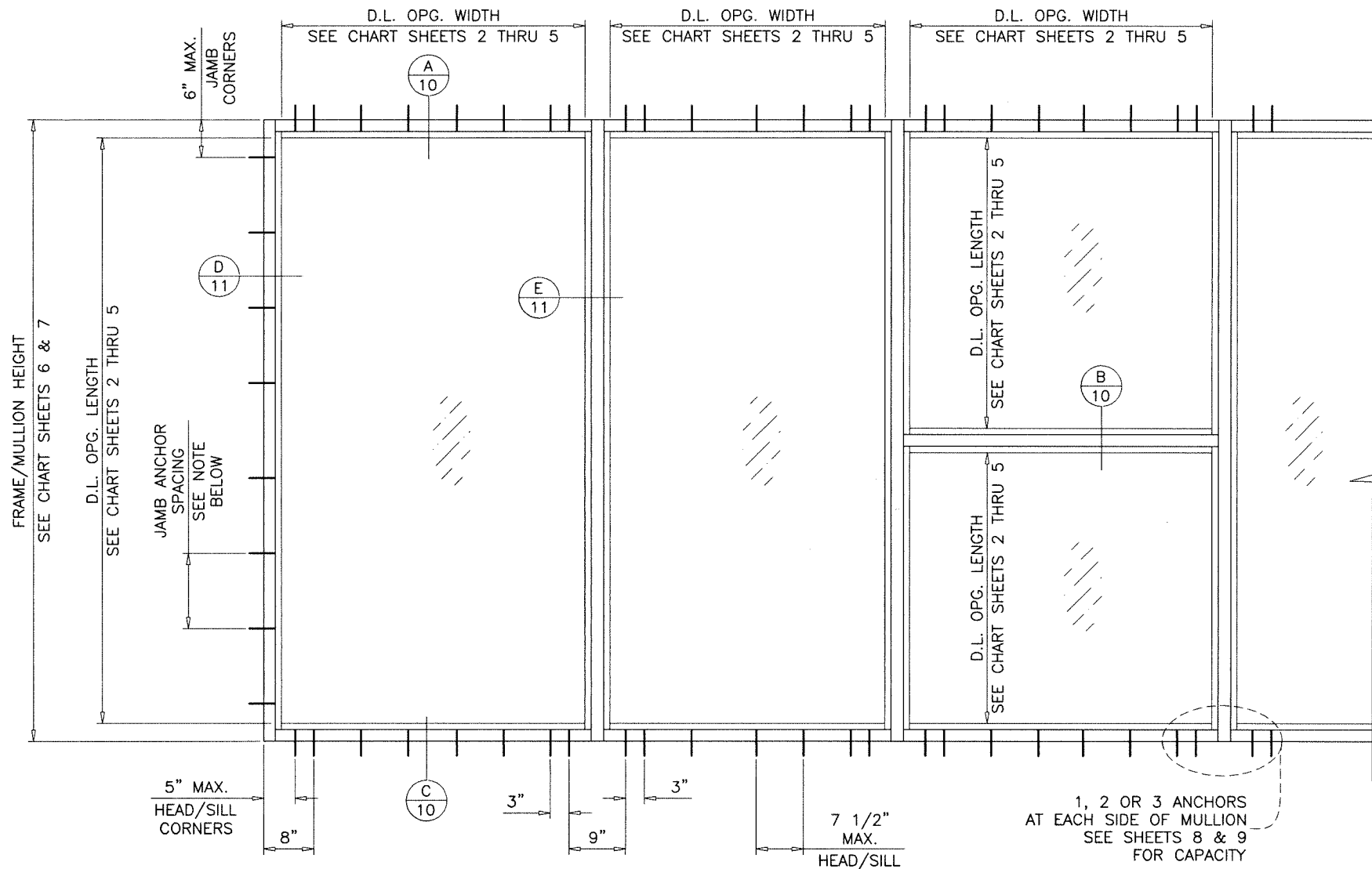
TYPICAL ELEVATIONS
