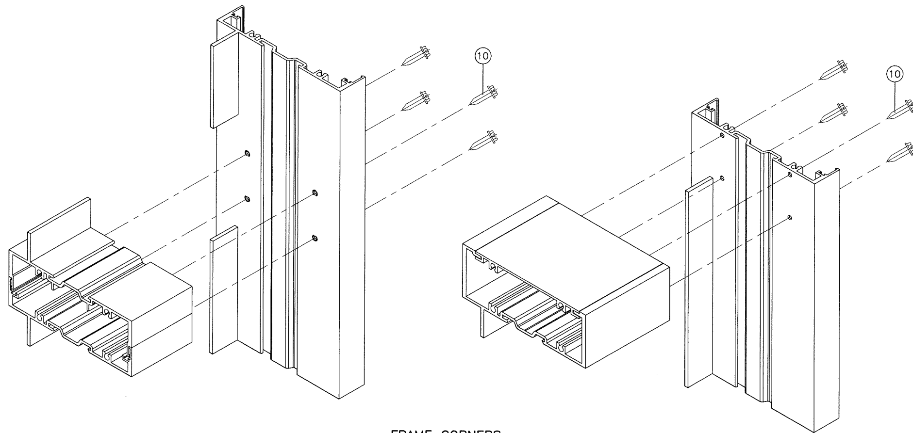
FRAME CORNERS
