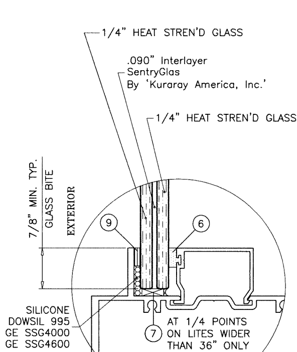
GLASS TYPE 'B' 9/16" OVERALL LAM. GLASS
