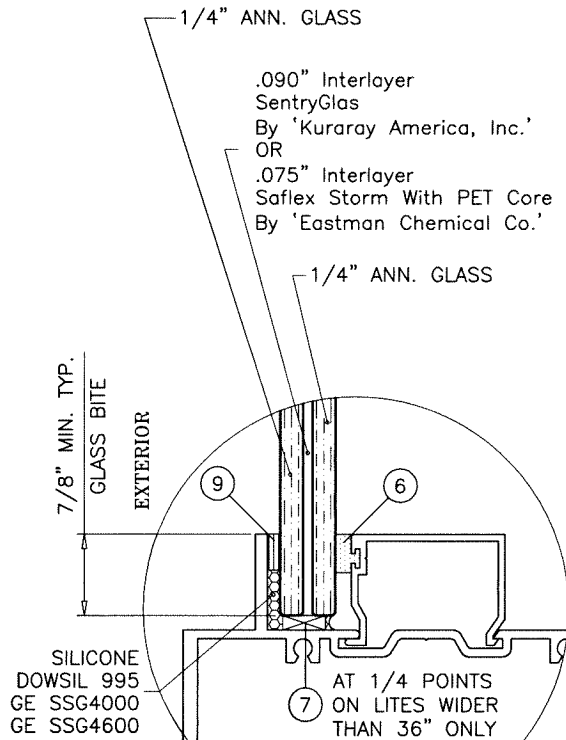
GLASS TYPE 'A' 9/16" OVERALL LAM. GLASS
