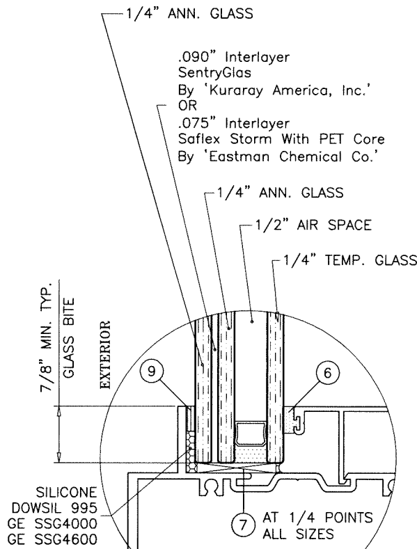
GLASS TYPE 'Ai' 1-3/8" OVERALL LAM. INSUL. GLASS
