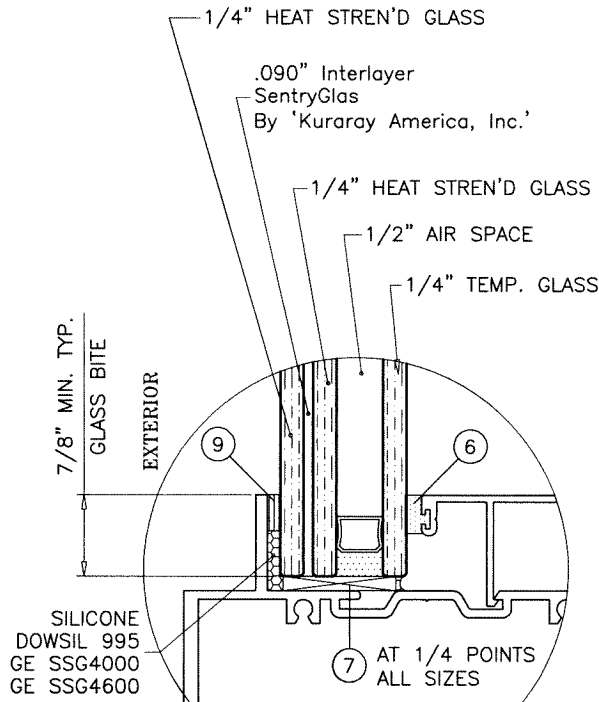
GLASS TYPE 'Bi' 1-3/8" OVERALL LAM. INSUL. GLASS
