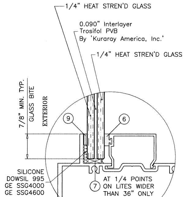
GLASS TYPE 'D' 9/16" OVERALL LAM. GLASS
