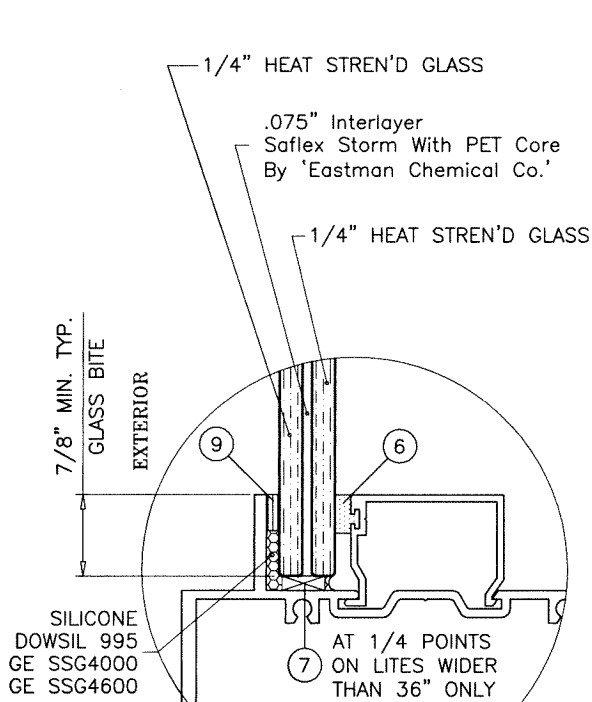
GLASS TYPE 'C' 9/16" OVERALL LAM. GLASS
