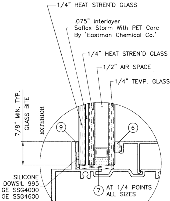
GLASS TYPE 'Ci' 1-3/8" OVERALL LAM. INSUL. GLASS
